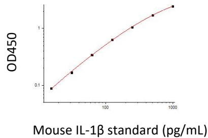
Fig.1. Standard Curve of Mouse IL-1 \beta in 96-well plate assay, data provided for demonstration purposes only. A new standard Curve must be generated for each assay
