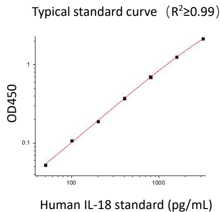
Fig.1. Standard Curve of Human IL-18 in 96-well plate assay, data provided for demonstration purposes only. A new standard Curve must be generated for each assay
